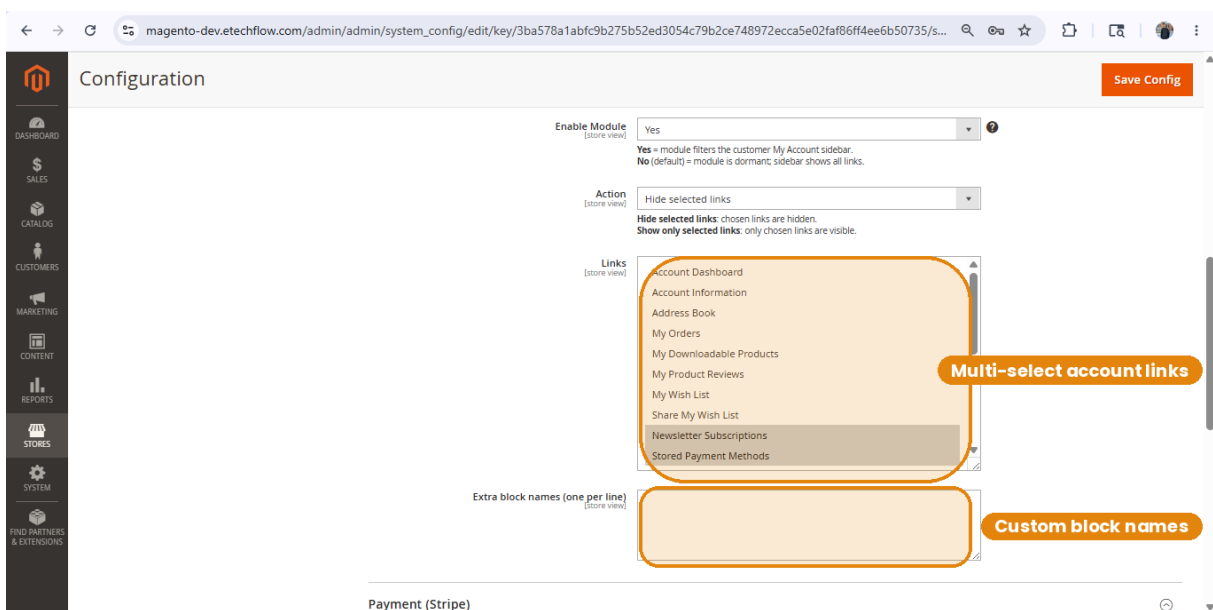
Figure 10 — The full Links multi-select showing every selectable account link, plus the optional "Extra block names (one per line)" field below for targeting custom sidebar blocks by name.
