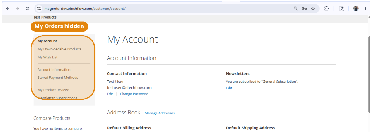
Figure 13 — Result of hiding My Orders: the sidebar now starts with My Account, My Downloadable Products, and My Wish List — no My Orders link is shown.
